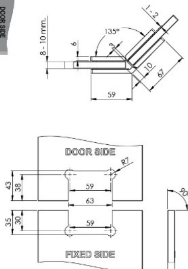
Glass cut option B: 90° fixed side
